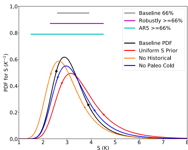
Figure 24. PDFs of S in comparison with AR5. The Baseline PDF is shown in black, and its 66% range (2.6–3.9 K) in gray. Colored curves show PDFs from sensitivity tests which cover a range for S , which could plausibly arise given reasonable alternative assumptions or interpretations of the evidence, summarized by the magenta line (2.3–4.5 K). These are the Baseline case but with a uniform S prior (red), the Baseline without the Historical evidence (orange), and the Baseline case without the cold paleoclimate evidence (blue). The 66%-or-greater (“likely”) range from the most recent IPCC assessment (AR5) (1.5–4.5 K) is shown in cyan. Circles indicate 17th and 83rd percentile values.
