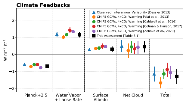
Figure 4. Estimates of global mean climate feedbacks from observations of interannual variability (blue triangles), from CMIP5 and CMIP6 model simulations of global warming in response to an abrupt \text{CO}_2 quadrupling (colored circles—orange: Vial et al., 2013; green: Caldwell et al., 2016; red: Colman & Hanson, 2017; and purple: Zelinka et al., 2020) and from this assessment (black squares). Error bars on climate model feedback estimates span the one standard deviation range across models. Observational estimates are derived using a combination of ERA-Interim meteorological fields and CERES TOA radiative fluxes (Loeb et al., 2009) covering the period March 2000 to December 2010 (Dessler, 2013). Error bars on the observational estimates are 1-sigma uncertainties, accounting for autocorrelation. Individual feedbacks are computed by multiplying temperature-mediated changes in relevant fields by radiative kernels (Huang et al., 2017; Shell et al., 2008; Soden et al., 2008). Error bars on values from this assessment correspond to 1-sigma uncertainties. Note that Planck feedback estimates are offset by 2.5 \text{ W m}^{-2} \text{ K}^{-1} from their actual values in order that they appear within the plot range.
