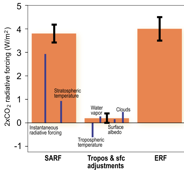
Figure 3. Assessed values of the 2\times\text{CO}_2 effective radiative forcing (ERF) at the TOA. Orange bars represent stratospheric-adjusted radiative forcing (SARF), tropospheric and surface albedo adjustments, and their sum (i.e., ERF). The error bar indicates the 5–95% ranges of the respective terms. Further decomposed components are presented for reference by blue bars based on Etminan et al. (2016) and Smith et al. (2018). The contribution from land surface warming has been excluded in the surface adjustment.
