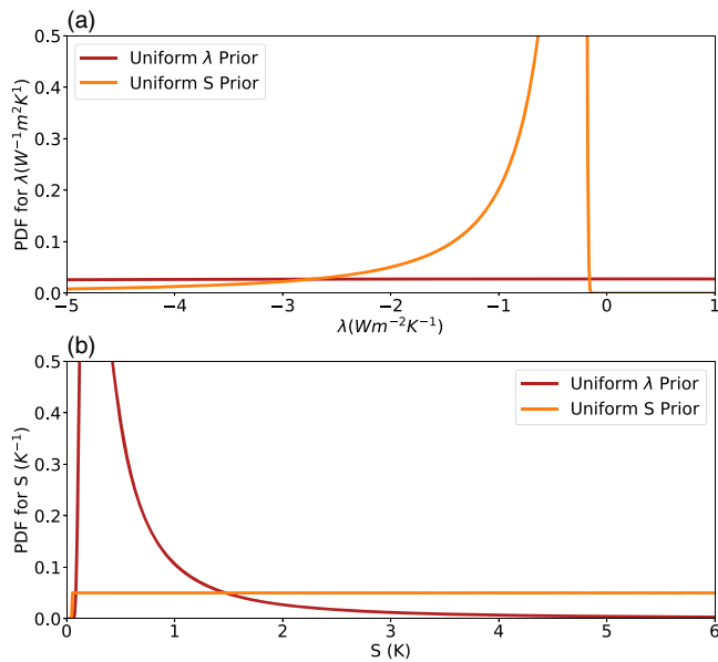
Figure 21. Prior predictive distributions for (a) \lambda and (b) S . Our Baseline (UL, red) prior is uniform in six \lambda_i feedbacks, each \sim U(-10, 10) \text{ W m}^{-2} \text{ K}^{-1} , compared to an alternative prior (US, orange), which reweights the Baseline prior to be uniform in S from near 0 to 20 K.
