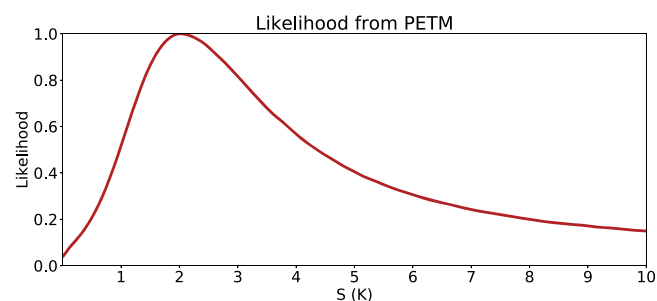
Figure 17. Likelihood arising for the Paleocene-Eocene Thermal Maximum. The maximum likelihood value of around 2 K corresponds to a 5-K warming and \sim 3\times\text{CO}_2 change together with its accompanying \text{CH}_4 increase.
