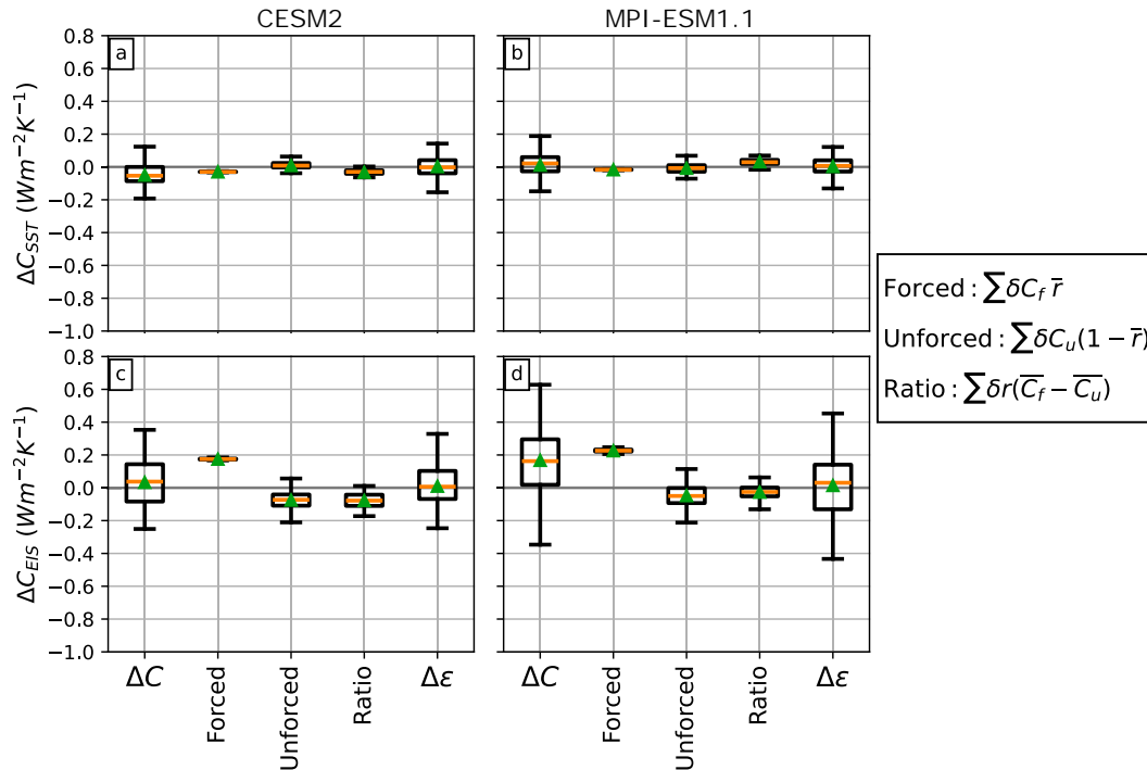
FIG. 3. As in Fig. 2, but for the \Delta C_{SST} decomposition between the 30-yr windows of 1981–2010 and 2070–99 in (a) CESM2 and (b) MPI-ESM1.1 and for the \Delta C_{EIS} decomposition between the 30-yr windows of 1981–2010 and 2070–99 in (c) CESM2 and (d) MPI-ESM1.1.
