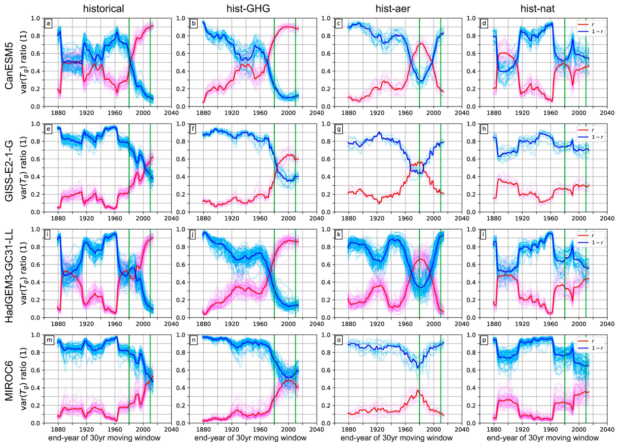
FIG. 7. Relative importance of the forced regressions r (red) and unforced regressions [(1 - r)] (blue) in (a) all-forcing LEs, (b) hist-GHG, (c) hist-aer, and (d) hist-nat experiments in CanESM5. Other rows are as in (a)–(d), but for (e)–(h) GISS-E2.1-G, (i)–(l) HadGEM3-GC3.1-LL, and (m)–(p) MIROC6. Dark-colored lines show the ensemble mean, and light-colored lines show individual ensemble members. (e) As in Fig. 1i.
