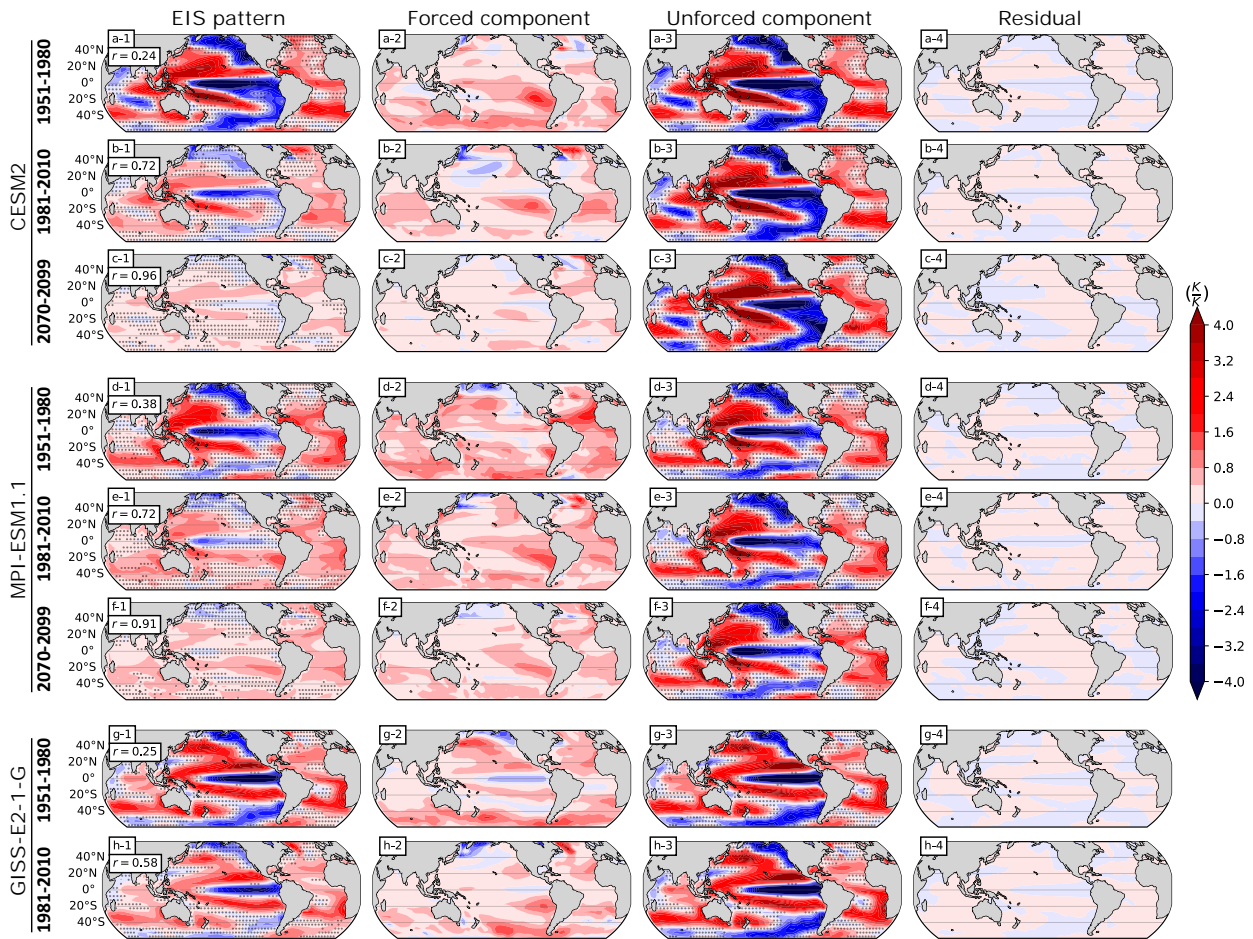
FIG. 5. As in Fig. 4, but for the overall EIS pattern dEIS/dT_g , the forced component dEIS_f/dT_{g,f} , the unforced component dEIS_u/dT_{g,u} , and the residual term \sigma calculated from each 30-yr window in each AOGCM LEs.
