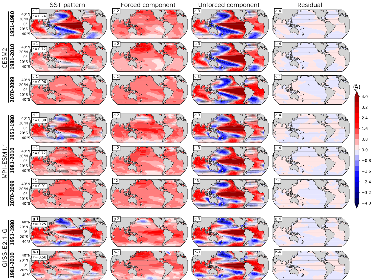
FIG. 4. (from left to right) Overall SST pattern dT/dT_g , the forced component dT_f/dT_{g,f} , the unforced component dT_u/dT_{g,u} , and the residual term \sigma calculated from different 30-yr windows in the three AOGCM LEs. For each panel, the 30-yr window and the LEs used are labeled on the left. In the overall and unforced SST patterns, contours indicate the ensemble mean and stippling indicates the regions where the one STD calculated across ensembles is larger than the ensemble-mean values. For the forced SST pattern, no stippling is shown since it is calculated based on the ensemble-mean fields before applying the OLS regression.
