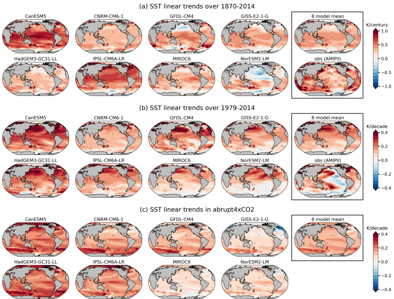
Figure 2. Historical and equilibrium SST trend patterns. Annual-mean SST linear trends over (a) 1870–2014, (b) 1979–2014, and (c) 150 years of abrupt-4xCO 2 simulations. The observed SST trend patterns in (a), (b) are calculated using AMIP2 dataset (Hurrell et al., 2008). Note that the color scales in (a) and (b) and (c) are different.
