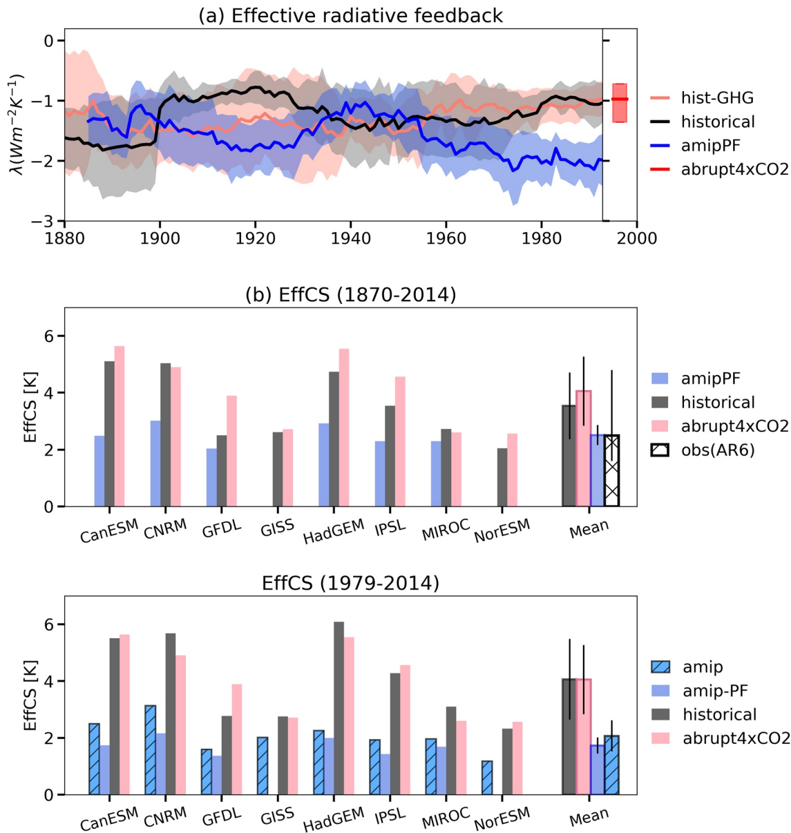
Figure 1. (a) Time series of the estimated \lambda_{his} . Thick lines denote multi-model means, shadings denote one standard deviation across models. The box plot on the right denotes the interquartile range (box) and the mean value (red line) of \lambda_{4xCO_2} across 8 models. (b and c) EffCS estimated from the energy budget of (b) full historical record (1870–2014) and (c) recent decades (1979–2014). The outlined colored bars on the right in (b), (c) denote the multi-model mean values of EffCS from corresponding simulations, with error bars indicating one standard deviation across models. The white hatched bar in (b) denotes the median EffCS his value of 2.5 K reported in AR6 (Forster et al., 2021) based on observed energy budget changes, with the error bars denoting 5%–95% range of 1.6–4.8 (k) Models listed (from the left to right) are: CanESM5, CNRM-CM6-1, GFDL-CM4, GISS-E2-1-G, HadGEM3-GC31-LL, IPSL-CM6A-LR, MIROC6, and NorESM2-LM.
