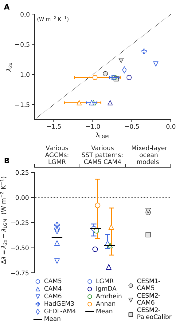
Fig. 2. LGM and 2xCO 2 climate feedbacks and LGM pattern effect ( \Delta\lambda ). Different AGCMs, all using the LGM R pattern for the LGM, are indicated by symbols; different LGM patterns (in CAM5 and CAM4) are indicated by colors. Error bars for Annan and LGM R represent first and fourth quartiles of ensemble members (Materials and Methods); central values indicate ensemble mean. For comparison with AGCM results using LGM data assimilation, the following feedbacks (in a mixed-layer ocean coupled to AGCM) from previous studies are also included: CESM1-CAM5 (23), CESM2-CAM6 (48), and CESM2-PaleoCalibr (49) (modified version of CAM6). (A) Scatterplot of 2xCO 2 feedbacks, \lambda_{2x} , versus LGM feedbacks, \lambda_{LGM} , with \lambda_{2x} = \lambda_{LGM} shown as dotted line. (B) LGM pattern effect, \Delta\lambda = \lambda_{2x} - \lambda_{LGM} , using feedbacks shown in (A), with \Delta\lambda = 0 shown as dotted line. Note that \Delta\lambda includes SST pattern effects and contributions from temperature dependence.
